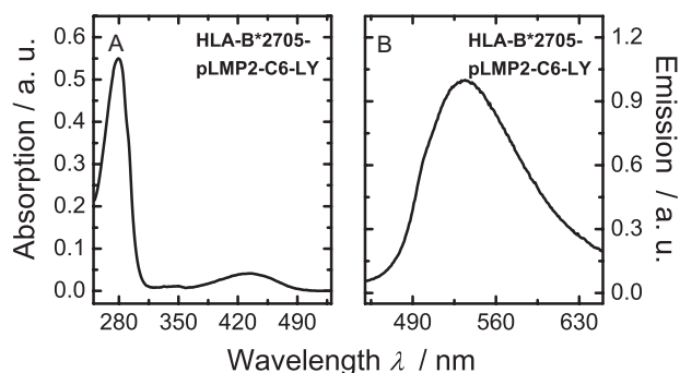
FIGURE 3. Absorption (A) and emission spectra (B) of the HLA-B*2705/pLMP2-C6-LY complex. Lucifer Yellow was excited at \lambda_{\text{ex}} = 428 nm. Conditions are as follows: 0.3 \mu\text{M} HLA-B27/peptide complex dissolved in 10 mM sodium phosphate buffer, 150 mM NaCl, pH 7.5.
