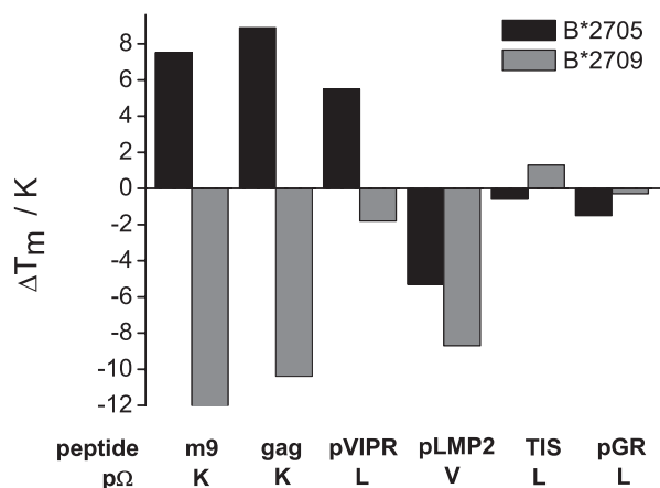
FIGURE 5. Transition temperatures for peptide dissociation ( T_m ) from the respective complexes with HLA-B*2705 and HLA-B*2709. The histogram shows the change in T_m ( \Delta T_m ) compared with T_m^* = 59\text{ }^\circ\text{C} (see text). The T_m values are taken from Table 2.
