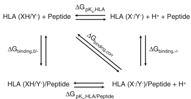
FIGURE 2. The general thermodynamic cycle used for the calculation of the peptide binding affinity. \Delta G_{\text{pK}_a,\text{HLA}/\text{Pep}} ( \Delta G_{\text{pK}_a,\text{HLA}} ) is the free energy difference associated with the deprotonation of the Glu-45/Glu-63 residue in the HLA-peptide complex (empty HLA molecule) (see Equation 6). To account for protonation changes of Glu-45/Glu-63 upon peptide binding, a corrected peptide binding affinity was used for the calculation: \Delta G_{\text{binding},\text{corr}} = \Delta G_{\text{binding}} + \Delta G_{\text{pK}_a,\text{X/Y}} denotes the Glu-45/63 pair.
