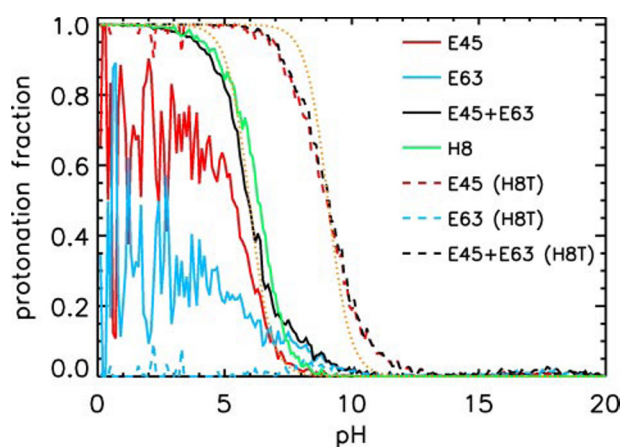
FIGURE 6. Protonation fraction of selected titratable groups (Glu-45, Glu-63, pHis-8) of HLA-B*2705 with bound pVIPR as a function of the pH value. The total protonation of Glu-45 and Glu-63 of B*2705 with bound pVIPR (mutated pVIPR-His8Thr) is denoted by a black line (black dashed line), and the respective Henderson-Hasselbalch fit by a dotted orange line.
