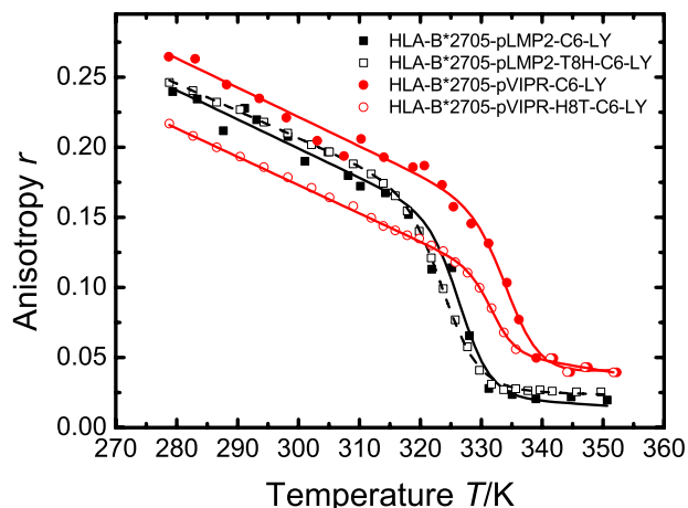
FIGURE 7. Steady state fluorescence anisotropy of HLA-B*2705/pLMP2-C6-LY (filled squares), HLA-B*2705/pLMP2-T8H-C6-LY (open squares), B*2705/pVIPR-C6-LY (filled circles), and HLA-B*2705/pVIPR-H8T-C6-LY (open circles) as a function of temperature. For B*2705 complexed with pLMP2-C6-LY and pVIPR-C6-LY, each data point represents the mean of five measurements. For B*2705 complexed with pLMP2-T8H-C6-LY and pVIPR-H8T-C6-LY, the temperature-dependent anisotropy curves are an average from two independent measurements. Conditions as in Fig. 3.
