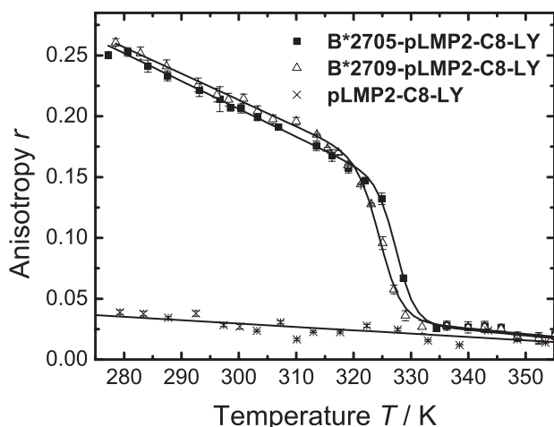
FIGURE 4. Steady state fluorescence anisotropy of HLA-B*2705/pLMP2-C8-LY (squares), B*2709/pLMP2-C8-LY (triangles), and the labeled peptide (crosses) as a function of temperature. Each data point represents the mean of five measurements. The S.E. is given. Conditions are as in Fig. 3.
