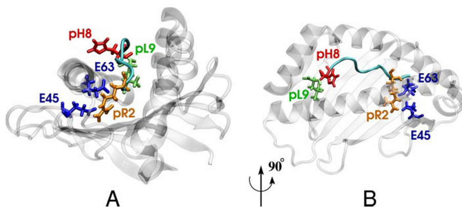
FIGURE 1. Peptide binding groove of HLA-B27 molecules. The pVIPR peptide (cyan) bound to B*2705 (gray) is shown. Glu-45, Glu-63 (blue), pArg-2 (yellow), pHis-8 (red), and pΩ (green) are emphasized in stick representation. B depicts the peptide binding groove as shown in A after a 90° rotation about the vertical axis.
