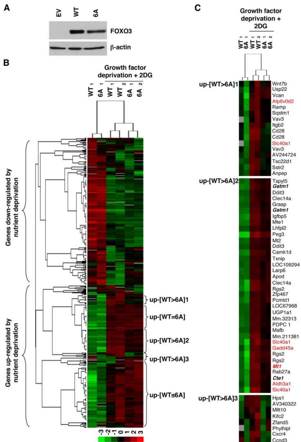
FIGURE 6. Genome-wide microarray identifies specific targets affected by AMPK phosphorylation of FOXO3. A , Foxo3 -/- MEFs were infected with retroviruses encoding empty vector (EV), FOXO3 WT, or 6A, and the levels of FOXO3 were assessed by Western blotting with an antibody to FOXO3 and to \beta -actin. B , FOXO3-rescued Foxo3 -/- MEFs were either left unstimulated or deprived of growth factors in the presence of 2DG (1 mM, 8 h). The genome-wide gene expression profiles in these samples were analyzed using Affymetrix Mouse Genome 420 arrays. The data presented correspond to one experiment conducted in duplicate (WT 1 or WT 2 and 6A 1 or 6A 2 ). Red, up-regulated gene expression; green, down-regulated gene expression; black, no change in gene expression; gray, probes that gave no reading. C , an unsupervised clustering analysis revealed three clusters containing genes that are more potently up-regulated in cells expressing FOXO3 WT than in cells expressing FOXO3 6A in response to nutrient deprivation (up-[WT > 6A]). Genes highlighted in red were verified by quantitative RT-PCR. Genes indicated in boldface and italic type were also identified in tissues from caloric restricted mice (52, 53).
