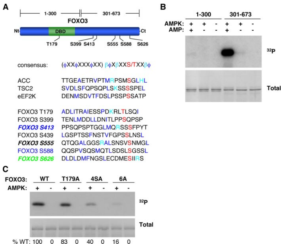
FIGURE 2. Identification of AMPK phosphorylation sites in FOXO3. A , location of the sites phosphorylated in vitro by AMPK in FOXO3. DBD , DNA binding domain. Alignments of the AMPK consensus phosphorylation motif with putative phosphorylation sites (in red) in human FOXO3 and sites in known substrates of AMPK. \phi , hydrophobic (dark blue); \beta , basic (light blue). The sites indicated in boldface and italic type were identified as being phosphorylated in vitro by AMPK by LC-MS/MS. The site indicated in green was identified as being phosphorylated in cells by LC-MS/MS. The sites indicated in blue were found to be phosphorylated in cells using phosphospecific antibodies. B , AMPK phosphorylates the C-terminal domain of FOXO3. The N-terminal (residues 1–300) or C-terminal (residues 301–673) domains of FOXO3 were incubated with purified AMPK in the presence of AMP and [ \gamma - ^{32} P]ATP. C , FOXO3 T179A mutant, quadruple mutant (S399A/S413A/S555A/S588A) (4SA), and sextuple mutant (T179A/S399A/S413A/S555A/S588A/S626A) (6A) display a reduction in phosphorylation by AMPK compared with WT FOXO3 in an in vitro kinase assay. The experiments presented in this figure are representative of at least two independent experiments.
