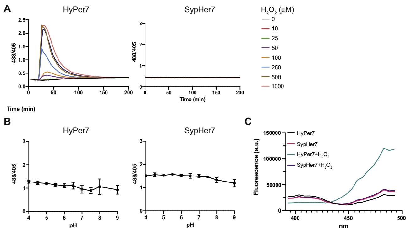
Figure 3. pH sensitivity of HyPer7 in yeast. A, response of BY4742 cells expressing HyPer7 (left panel) or SypHer7 (right panel) to exogenously applied H 2 O 2 bolus in the concentration range of 10 to 1000 μM. B, response of BY4742 cells expressing HyPer7 (left panel) or SypHer7 (right panel) to exogenously applied pH buffers in the range between 4 and 9. C, fluorescence excitation spectra (emission: 520 nm) of yeast cells expressing HyPer7 or SypHer7, collected at pH 6. Cells were left untreated or treated with 10 mM H 2 O 2 . Data in this figure are representative of n = 3 independent experiments with n = 3 independent replicates each.
