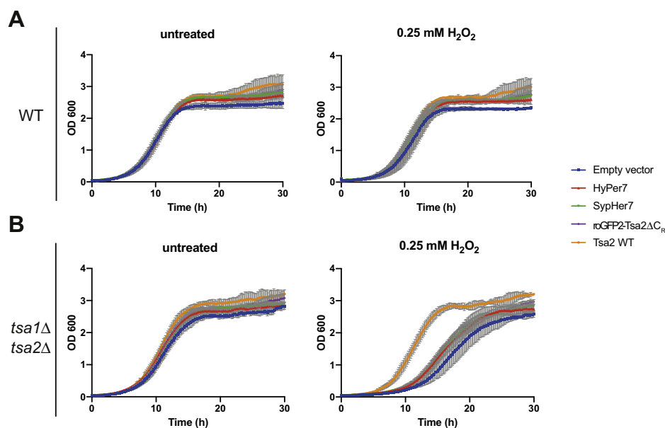
Figure 5. Influence of the probes on cell growth and endogenous H 2 O 2 scavenging. A , growth curve of a WT BY4742 strain transformed with an empty vector, Tsa2 WT, roGFP2-Tsa2ΔC R , HyPer7, or SypHer7. The cells were exposed to 0.25 mM of H 2 O 2 2 h after the start of the experiment. B , growth curve of a tsa1 Δ tsa2 Δ strain transformed with an empty vector, Tsa2 wt, roGFP2-Tsa2ΔC R , HyPer7, or SypHer7. The cells were exposed to 0.25 mM of H 2 O 2 2 h after the start of the experiment.
