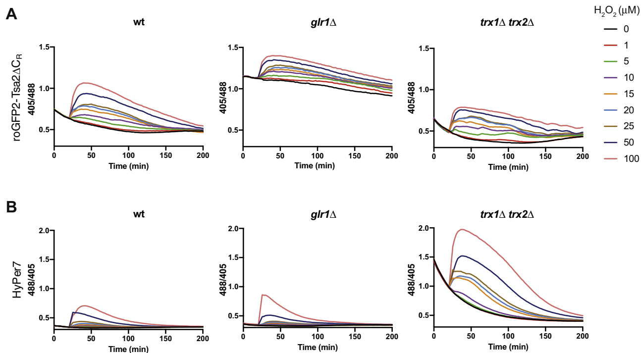
Figure 4. Influence of thiol-reducing systems on cytosolic HyPer7. A , response of WT ( left panel ), Glr1-deficient ( middle panel ), and Trx1/Trx2-deficient ( right panel ) BY4742 cells expressing roGFP2-Tsa2ΔC R to a range of different H 2 O 2 concentrations (0–100 μM). B , response of WT ( left panel ), Glr1-deficient ( middle panel ), and Trx1/Trx2-deficient ( right panel ) BY4742 cells expressing HyPer7 to a range of different H 2 O 2 concentrations (0–100 μM). Data in this figure are representative of n = 3 independent experiments with n = 3 independent replicates. Trx, thioredoxins.
