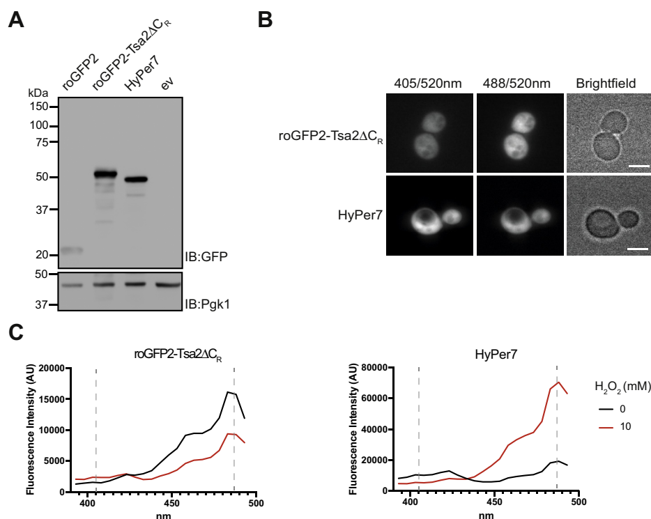
Figure 1. Expression of HyPer7 in yeast. A, expression of roGFP2, roGFP2-Tsa2ΔC R , and HyPer7 under the TEF promoter in the WT BY4742 strain. Immunoblotting with anti-GFP and anti-Pgk1 antibodies. B, fluorescence (520 nm) emitted by WT BY4742 yeast cells expressing either roGFP2-Tsa2ΔC R (upper panels) or HyPer7 (lower panels), after excitation at 405 (left panels) and 488 nm (middle panels). The scale bar represents 4 μm. C, fluorescence excitation spectra (emission: 520 nm) of yeast cells expressing roGFP2-Tsa2ΔC R (left panel) or HyPer7 (right panel). Cells were left untreated (black line) or treated with 10 mM H 2 O 2 (red line). Dashed vertical lines indicate the position of the 405- and 488-nm laser lines. Data in this figure are representative of n = 3 independent experiments with n = 3 independent replicates each. ev, empty vector.
